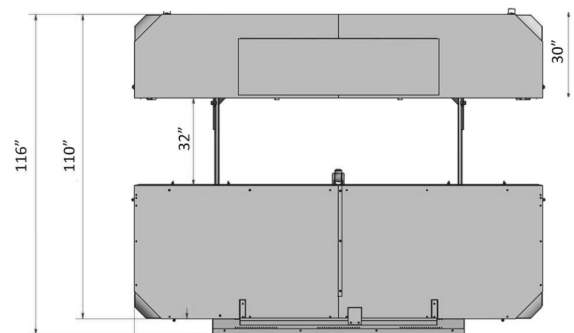
Top View Servicing
